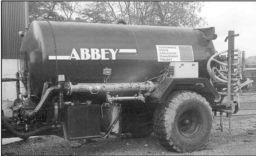
Plate 1. The assembled prototype tanker.
