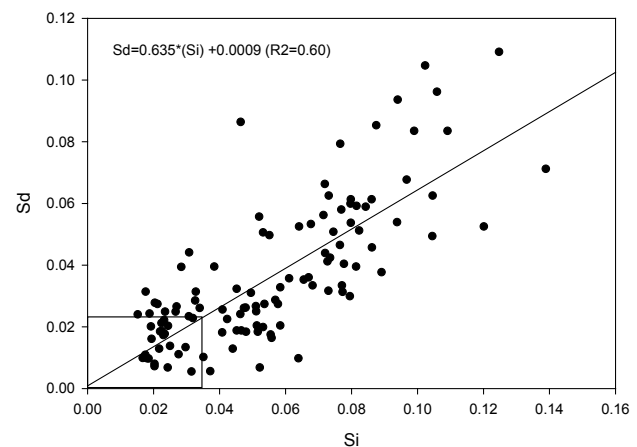
Figure 2. S -Indirect ( S_i ) versus S -Direct ( S_o ) S -term for all soil horizons. For example, an S_i value of 0.035 (degradation threshold) equates to an S_o of 0.023 (below threshold). This includes all data from Table 2.
