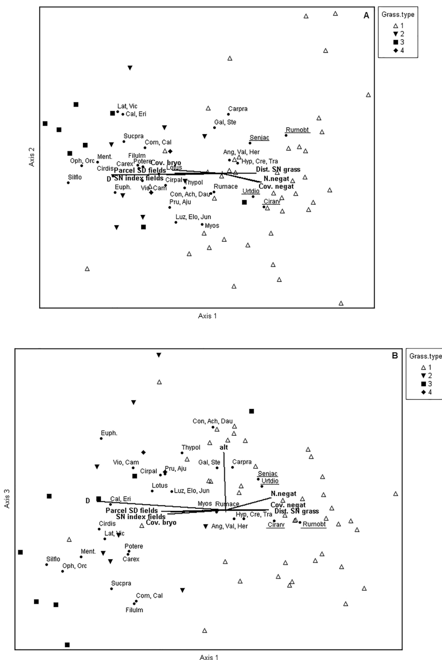
Fig. 2. NMS ordination plots showing the relationship between indicator species composition and environmental variables in relation to NMS axes (grasslands). Only species that have correlations above |0.300| are identified (dots). Graph A: Axis 1 plotted against Axis 2; Graph B: Axis 1 plotted against Axis 3. Legend for “Grass.type”: improved grasslands = 1; semi-improved grasslands = 2; semi-natural grasslands = 3; transition to semi-natural grasslands = 4. Species names can be consulted in Table S1 in the Supplementary Materials and Table S9 shows all correlation values between species and ordination axes. Negative indicator species are underlined.
