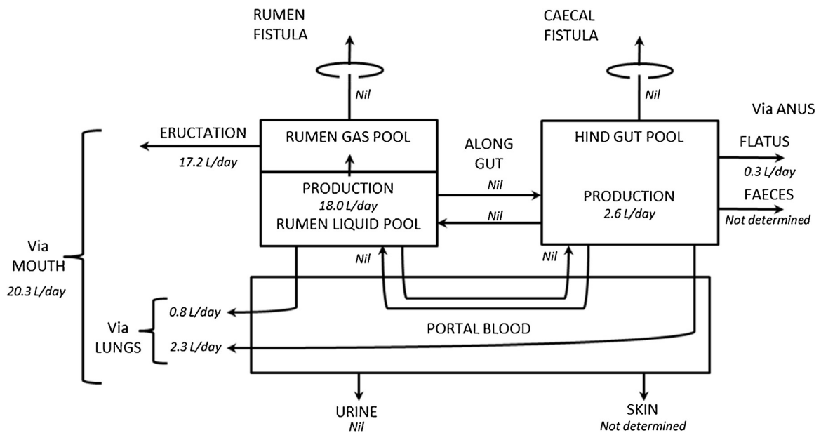
Fig. 1. A model of the production and movement of methane in sheep on a lucerne chaff diet. Diagram sourced from Murray et al. (1975).
