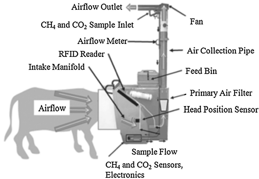
Fig. 3. Layout of the GreenFeed system (C-Lock Inc., Rapid City, SD, USA). Sourced from Huhtanen et al. (2015).
