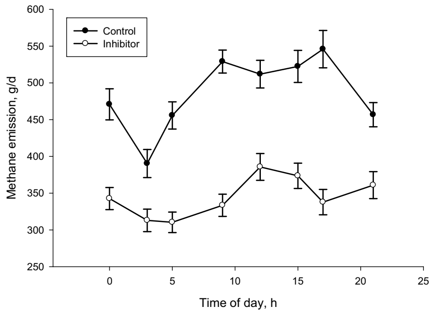
Fig. 5. Methane emission by lactating dairy cows ( n = 12 for control and n = 36 for treatment) fed a total mixed ration without (control) or with (inhibitor) 3-nitroxypropanol. Sourced from Hristov et al. (2015b) .
