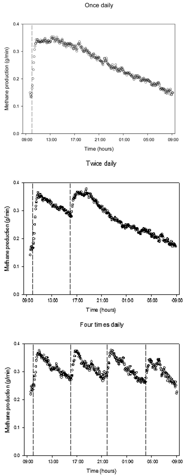
Fig. 4. Diurnal pattern of methane emission (mean of three daily measurements for 4 animals) by lactating dairy cows fed the same total mixed ration once, twice, or four times daily. Dotted lines indicate the time of feeding. Sourced from Crompton et al. (2011) .
